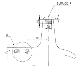
POSITION FOR TAKING TEST SPECIMEN
